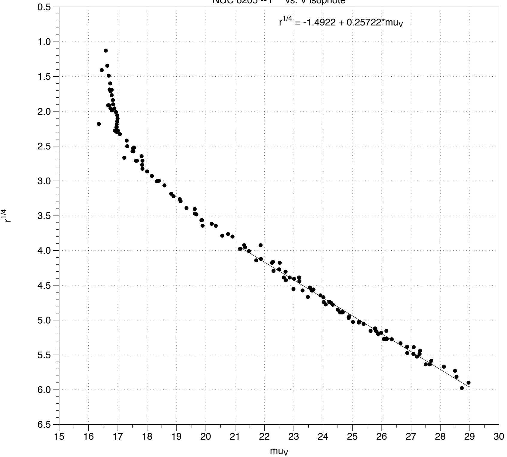
NGC 6205 -- r^{1/4} vs. V isophote
