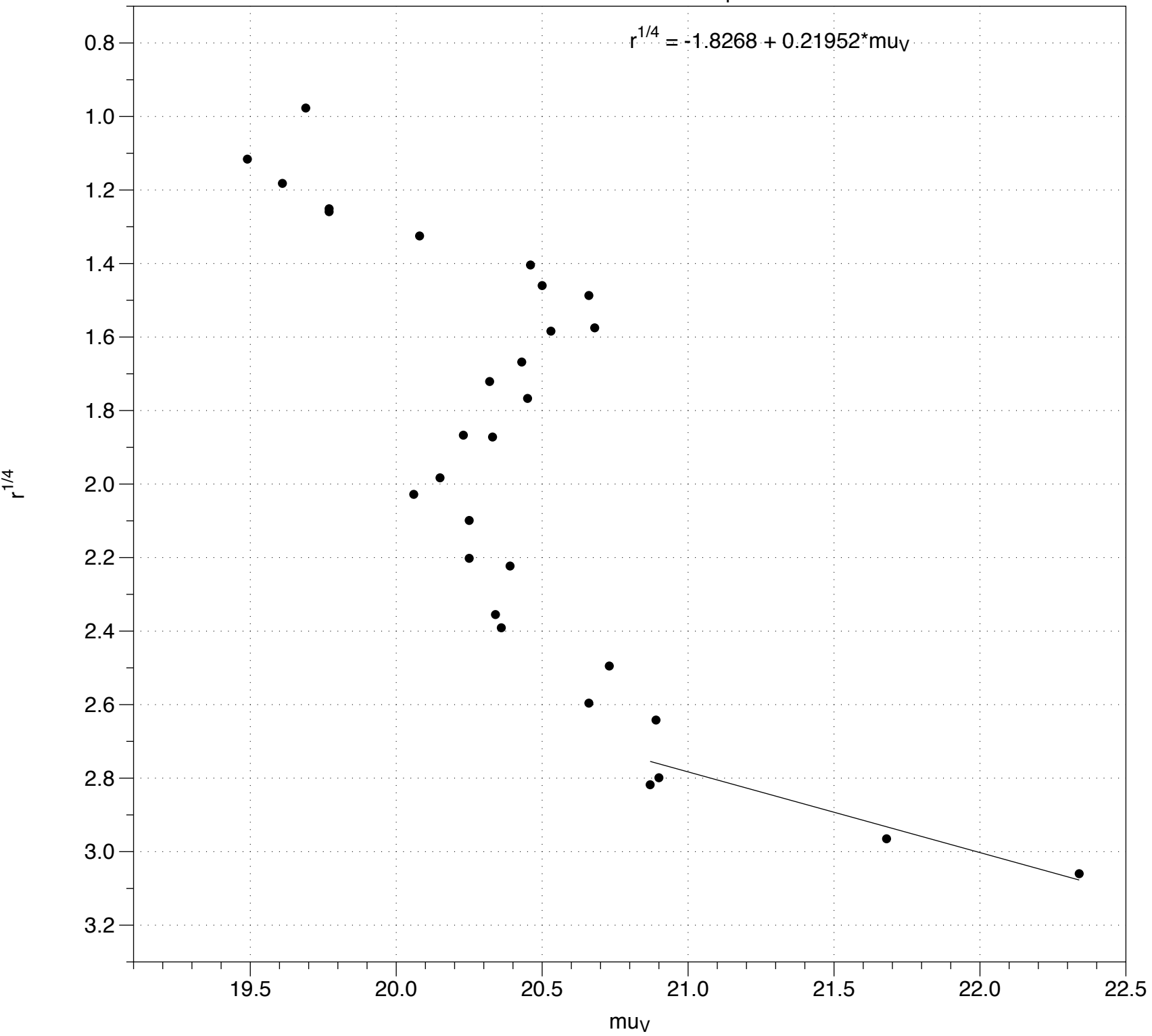
NGC 6496 -- r^{1/4} vs. V isophote
