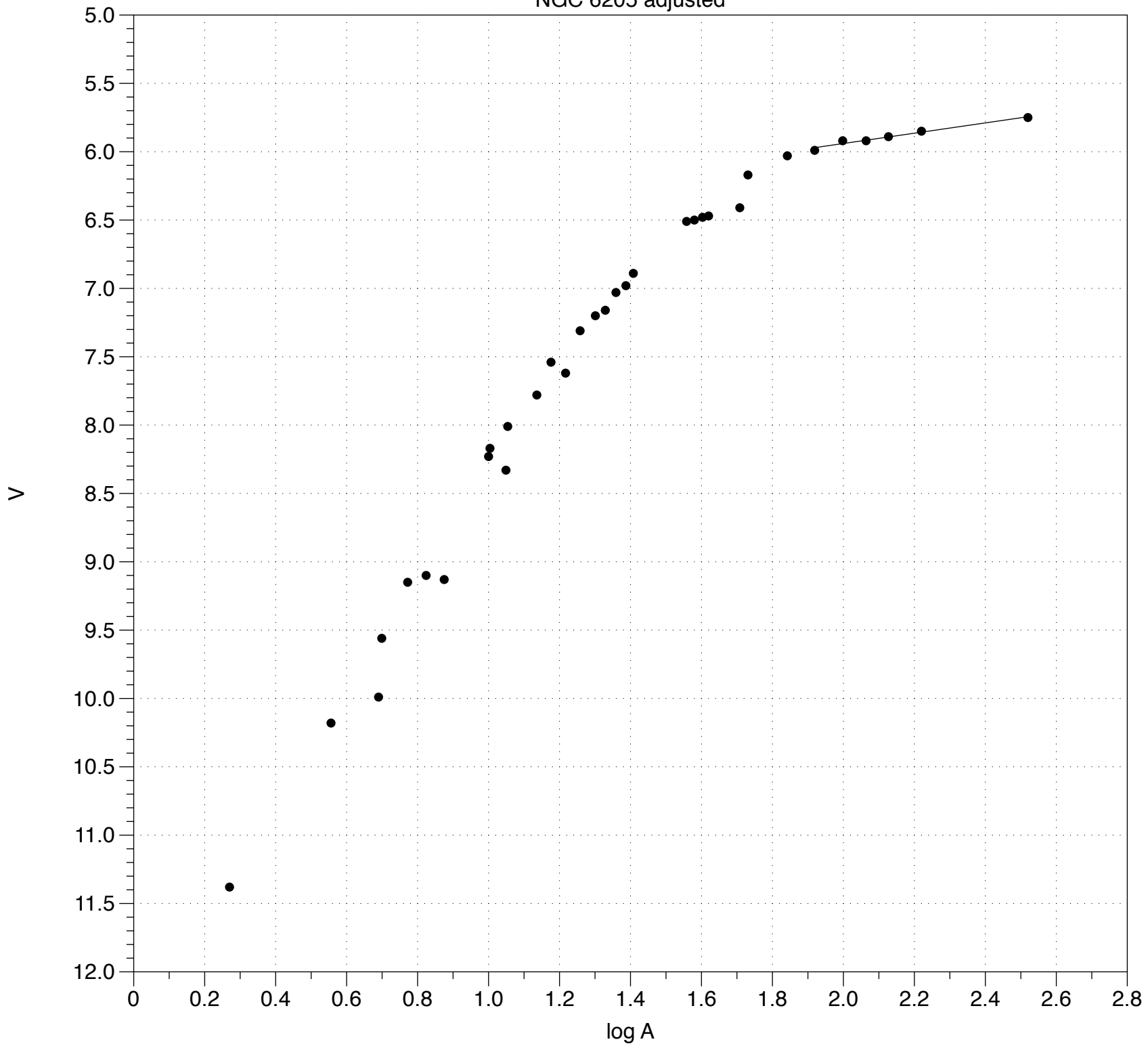
NGC 6205 adjusted
