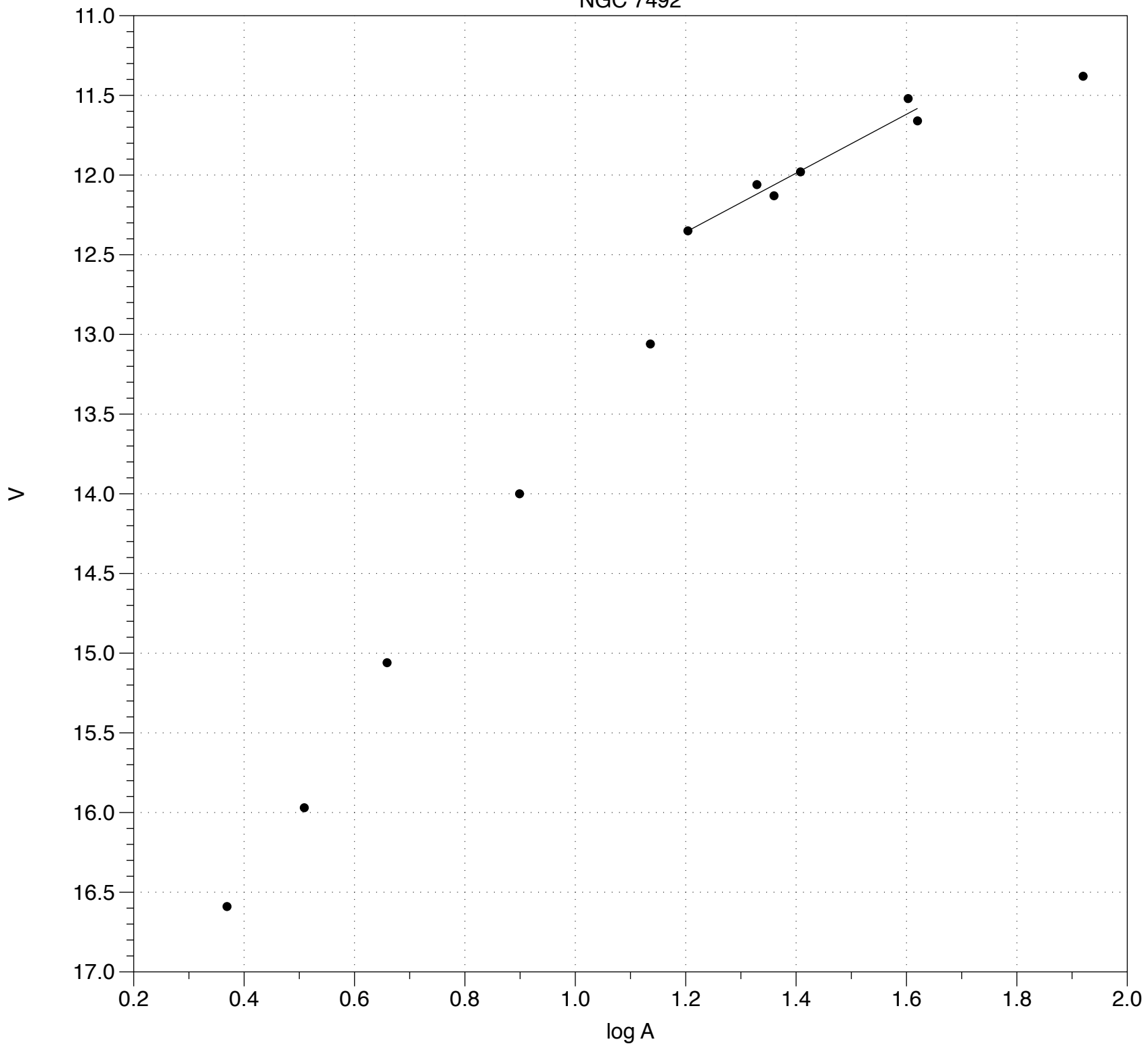
NGC 7492
