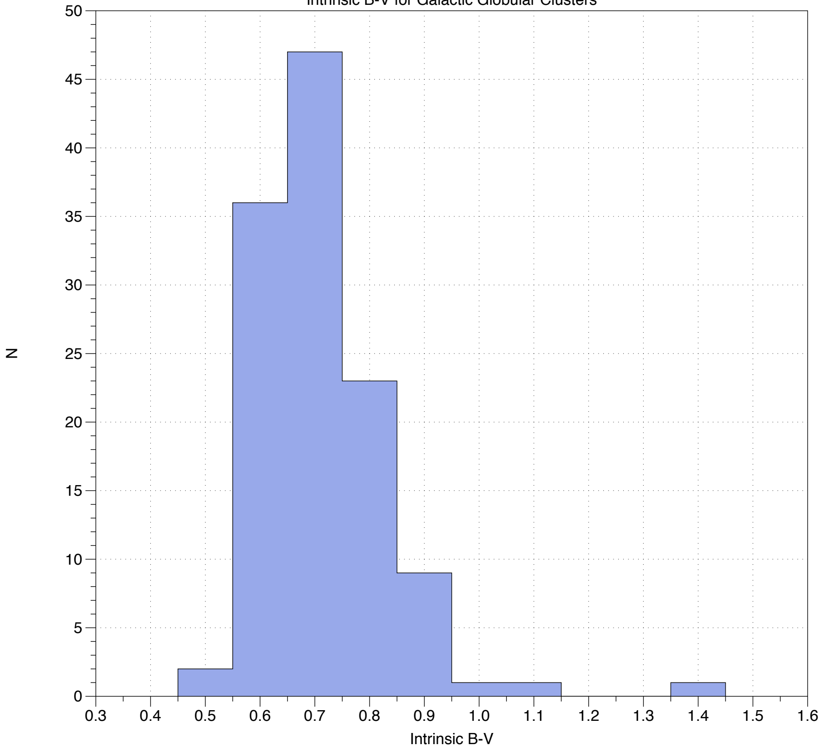
Intrinsic B-V for Galactic Globular Clusters
