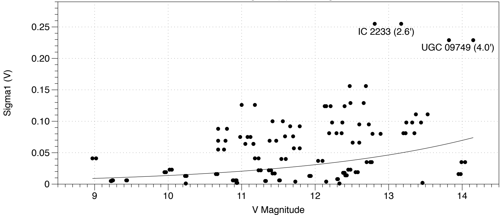
Galaxies: Sigma1 (V) vs. V Magnitude
