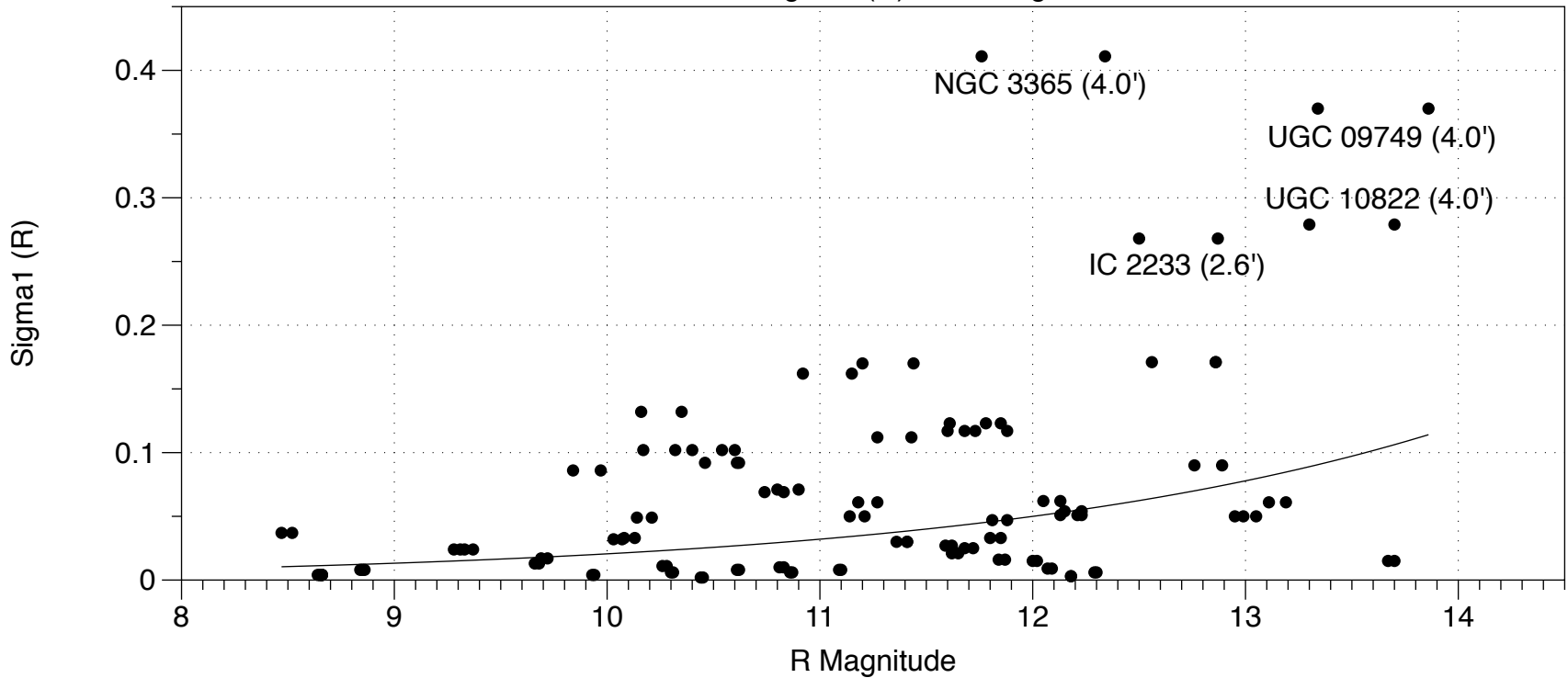
Galaxies: Sigma1 (R) vs. R Magnitude
