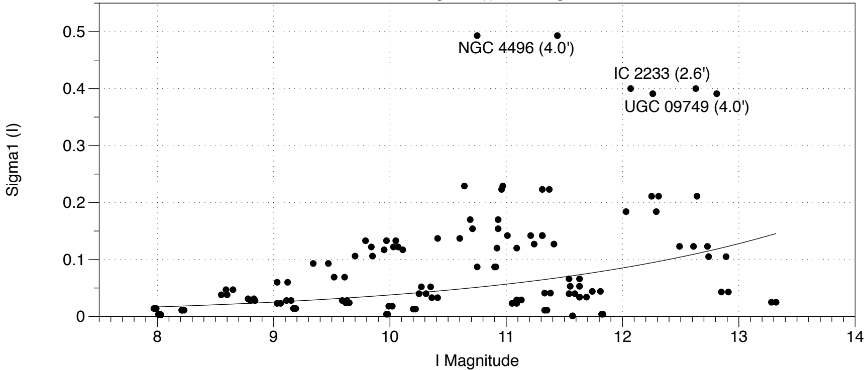
Galaxies: Sigma1 (I) vs. I Magnitude
