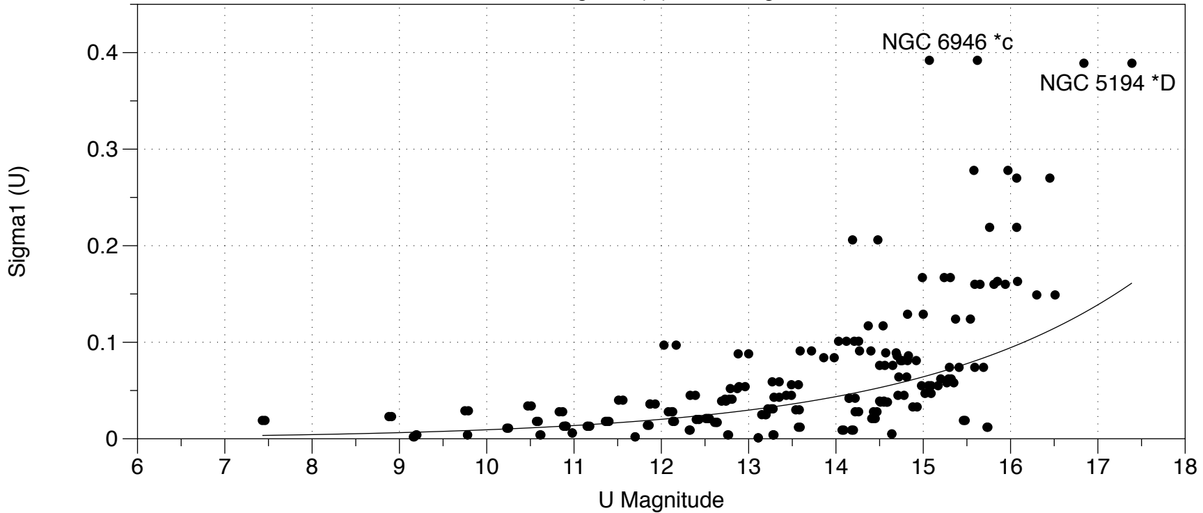
Stars: Sigma1 (U) vs. U Magnitude
