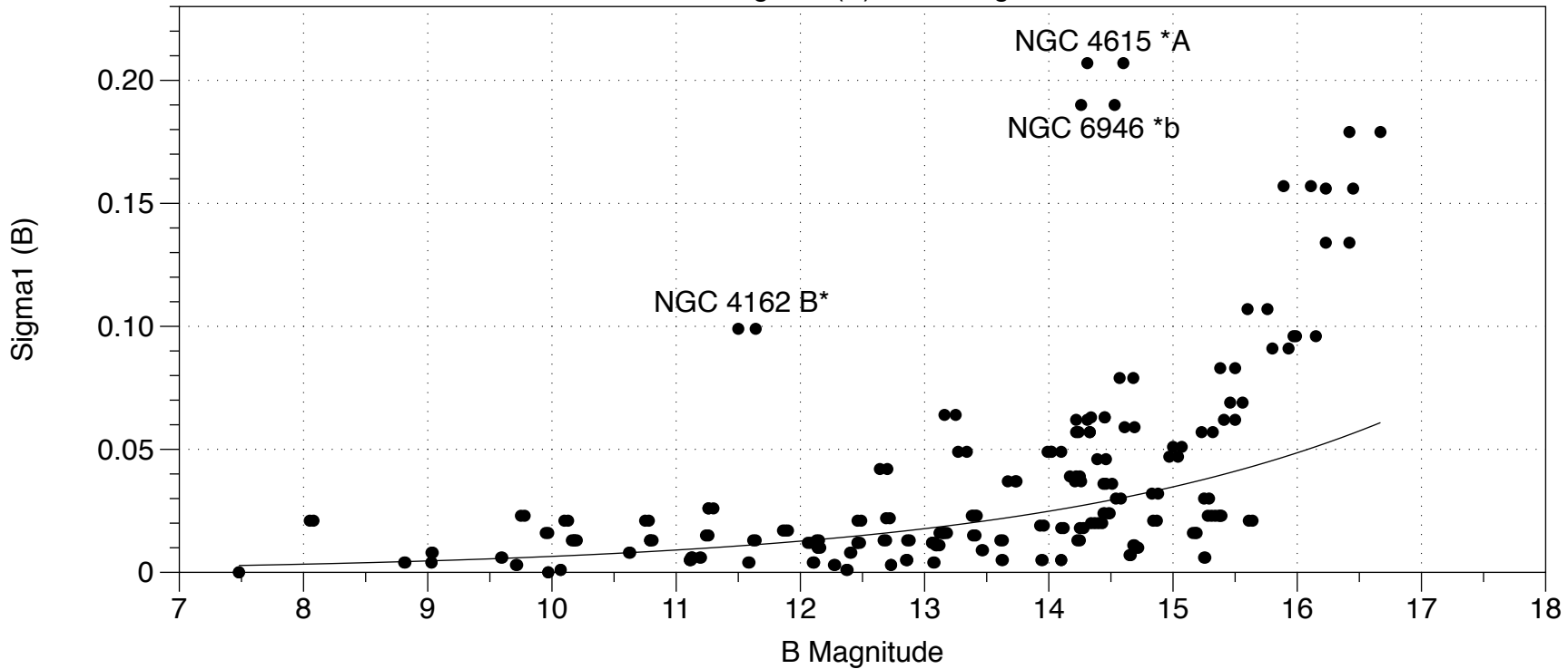
Stars: Sigma1 (B) vs. B Magnitude
