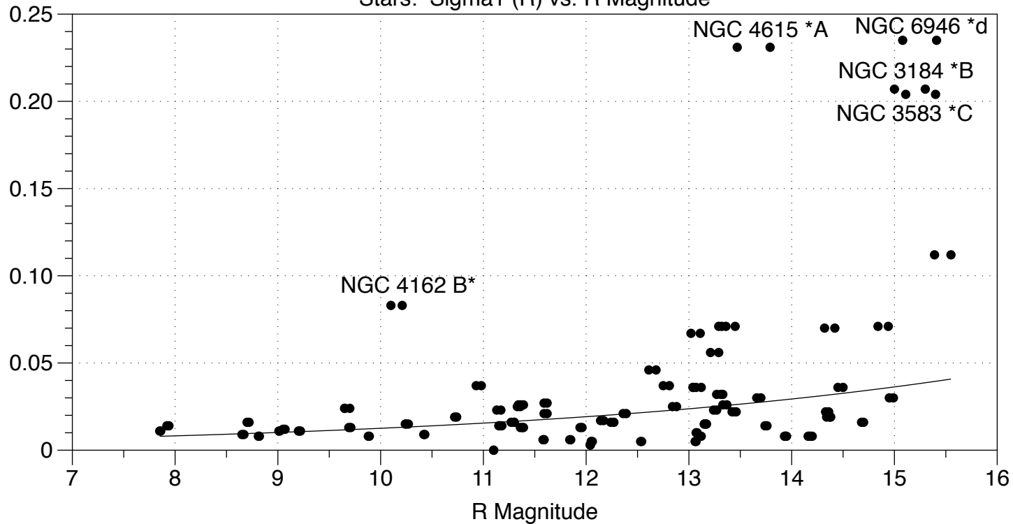
Stars: Sigma1 (R) vs. R Magnitude
