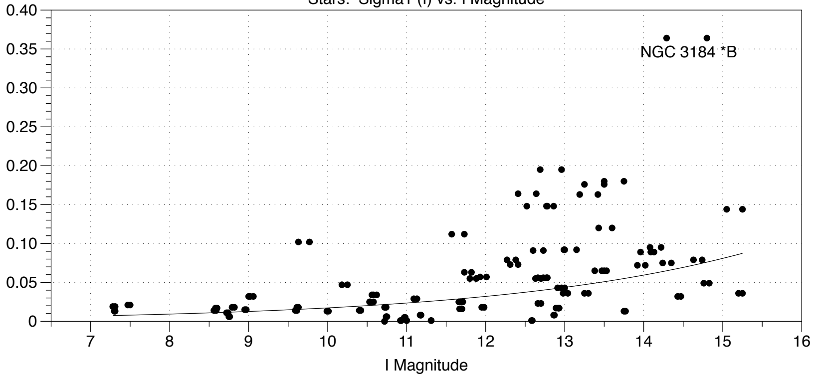
Stars: Sigma1 (I) vs. I Magnitude
