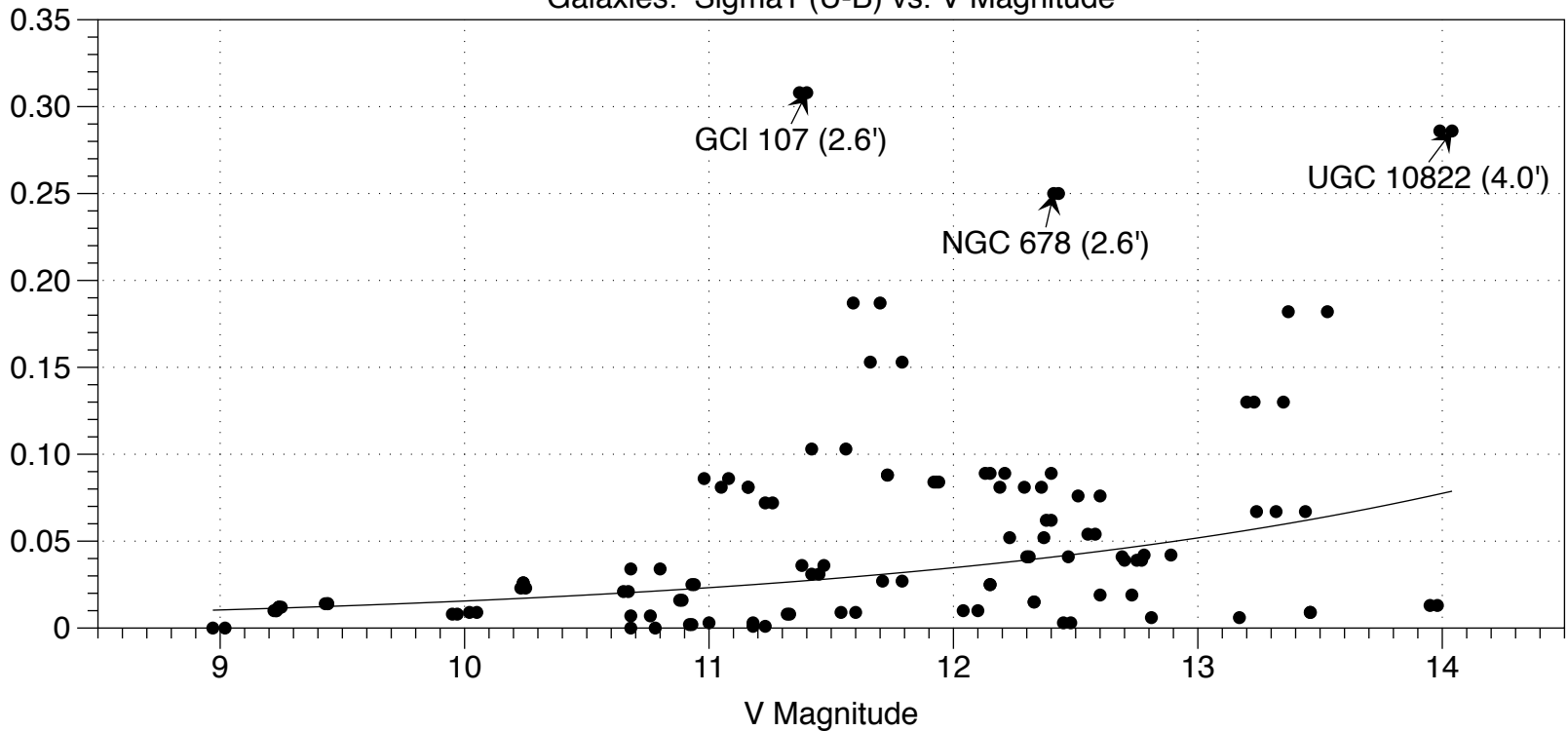
Galaxies: Sigma1 (U-B) vs. V Magnitude
