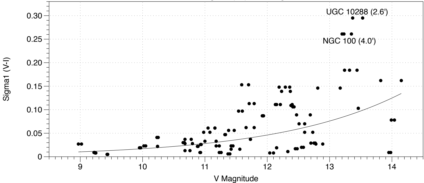
Galaxies: Sigma1 (V-I) vs. V Magnitude
