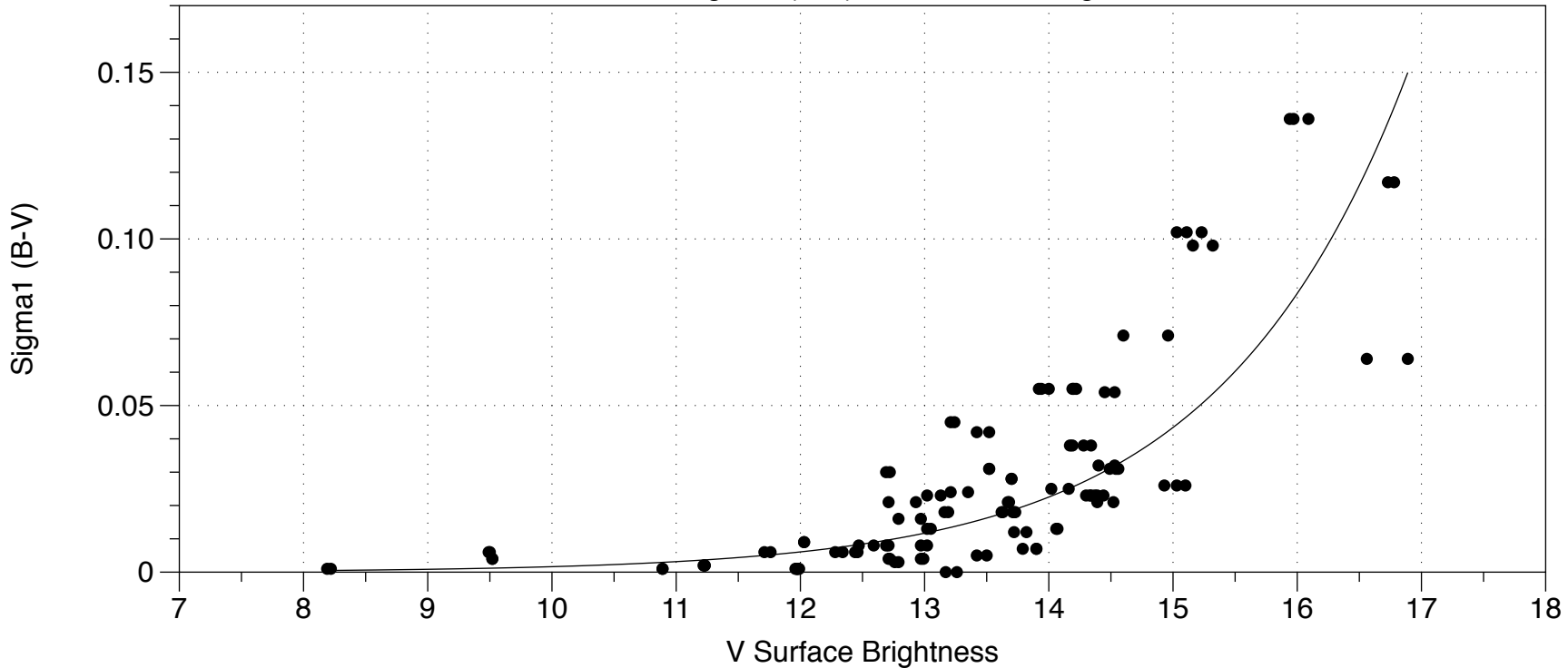
Galaxies: Sigma1 (B-V) vs. V Surface Brightness
