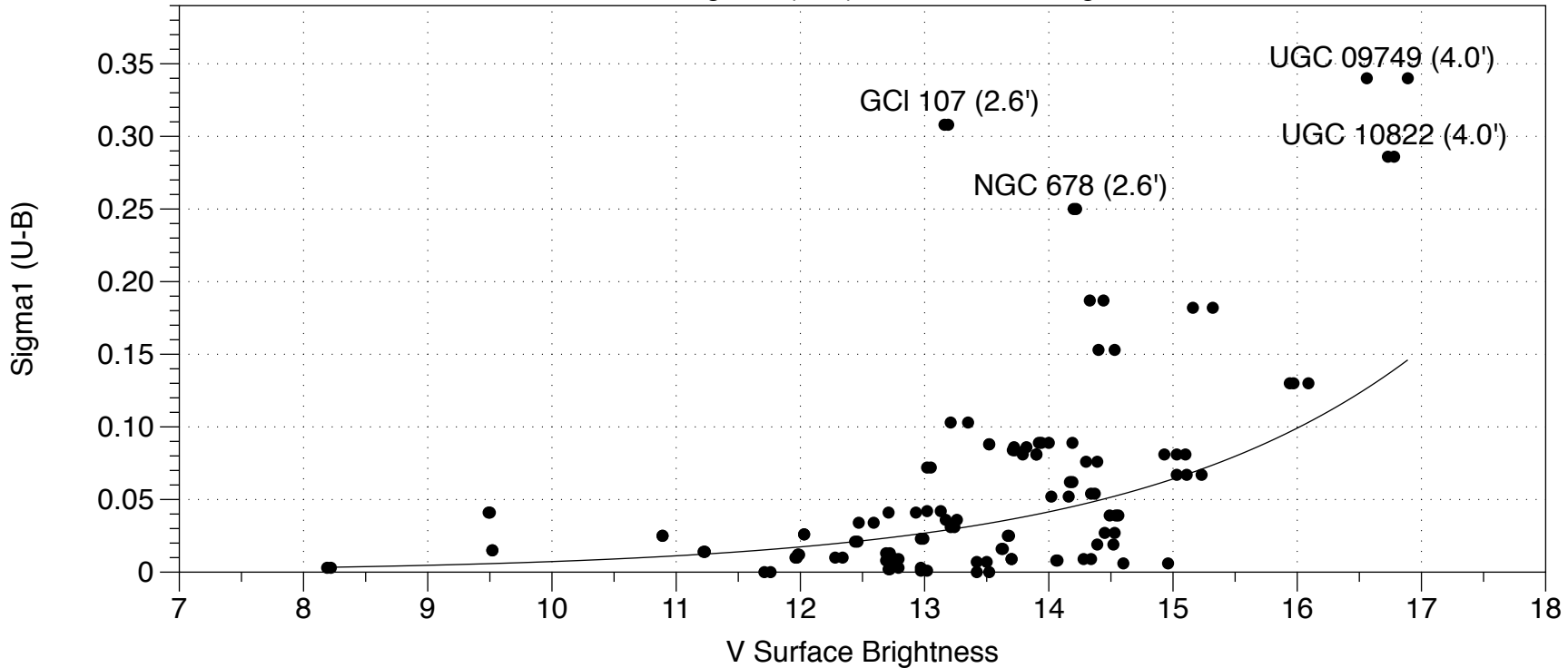
Galaxies: Sigma1 (U-B) vs. V Surface Brightness
