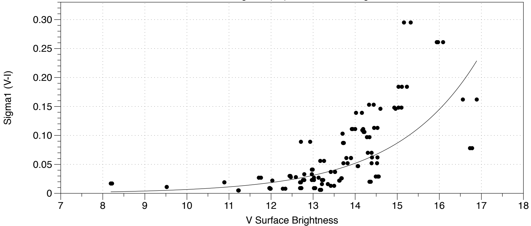
Galaxies: Sigma1 (V-I) vs. V Surface Brightness
