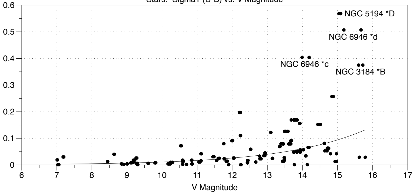
Stars: Sigma1 (U-B) vs. V Magnitude
