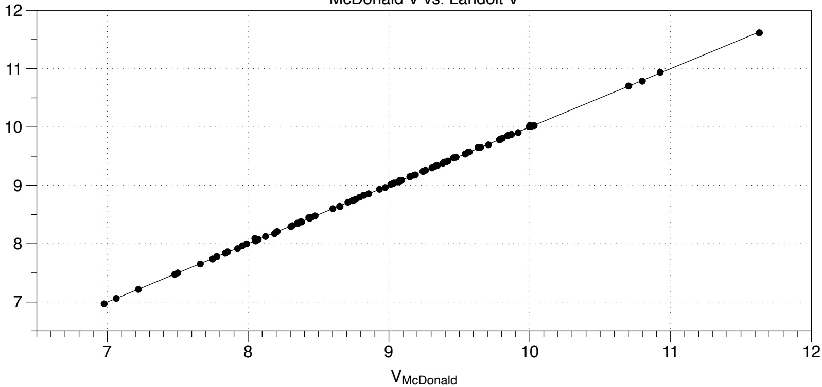
McDonald V vs. Landolt V
