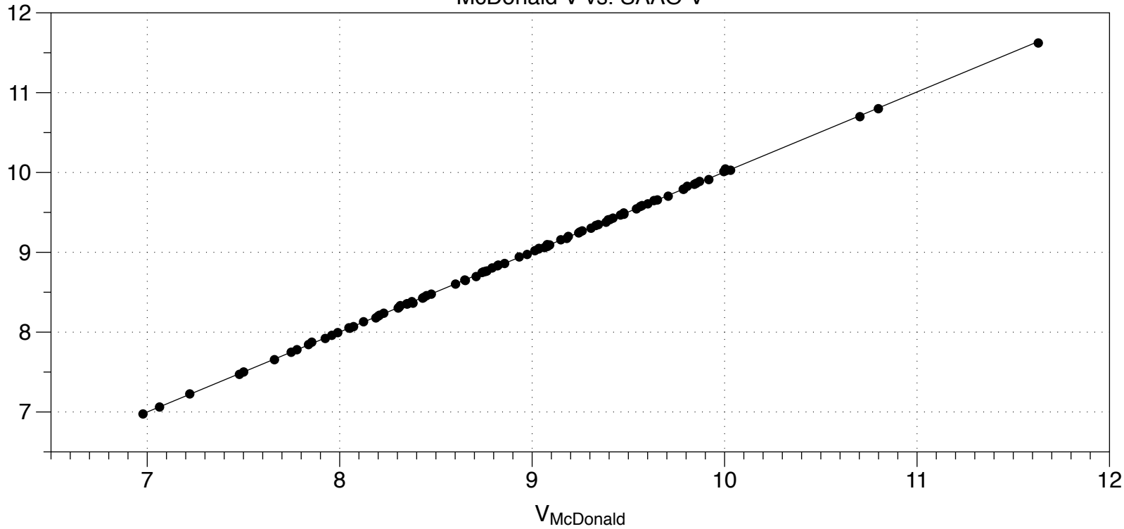
McDonald V vs. SAAO V
