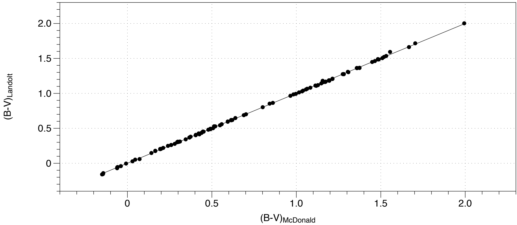
McDonald B-V vs. Landolt B-V
