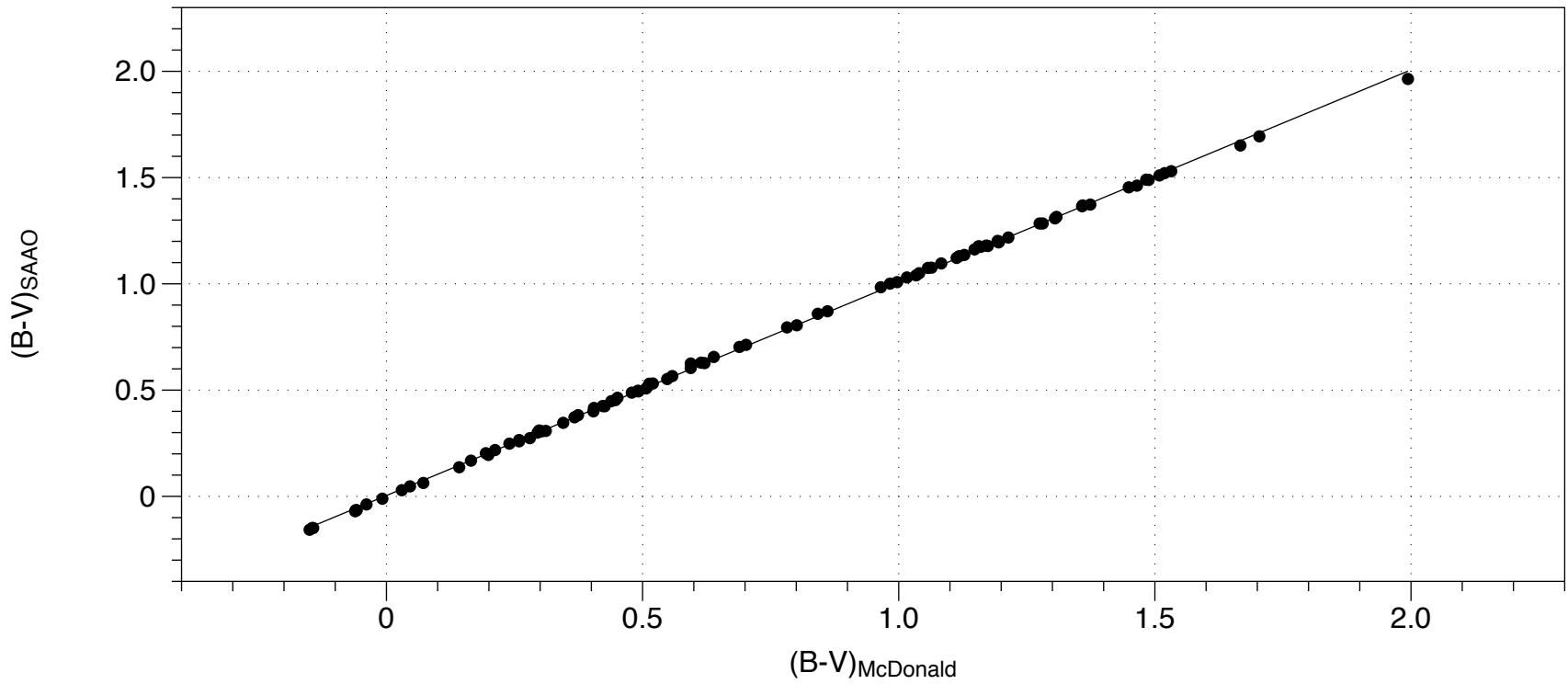
McDonald B-V vs. SAAO B-V
