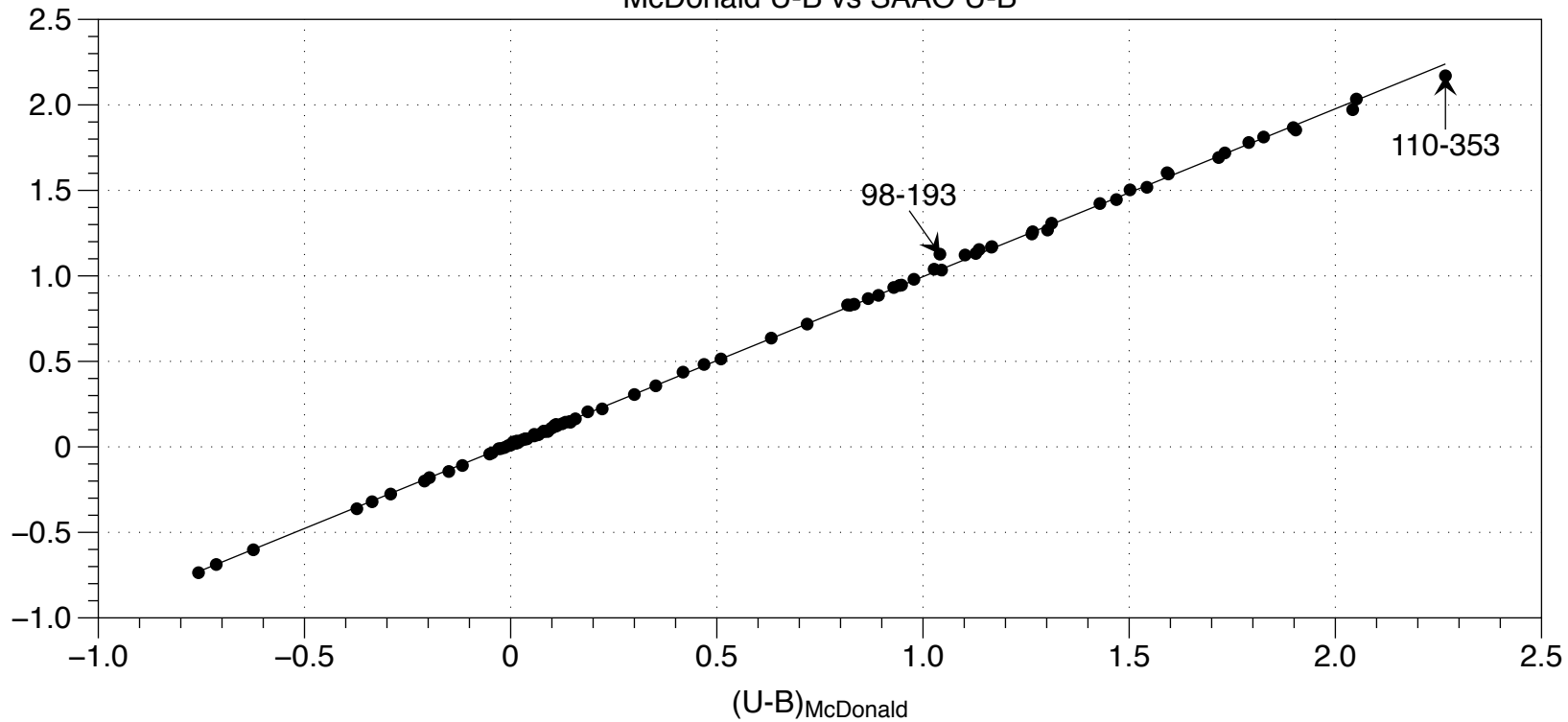
McDonald U-B vs SAAO U-B
