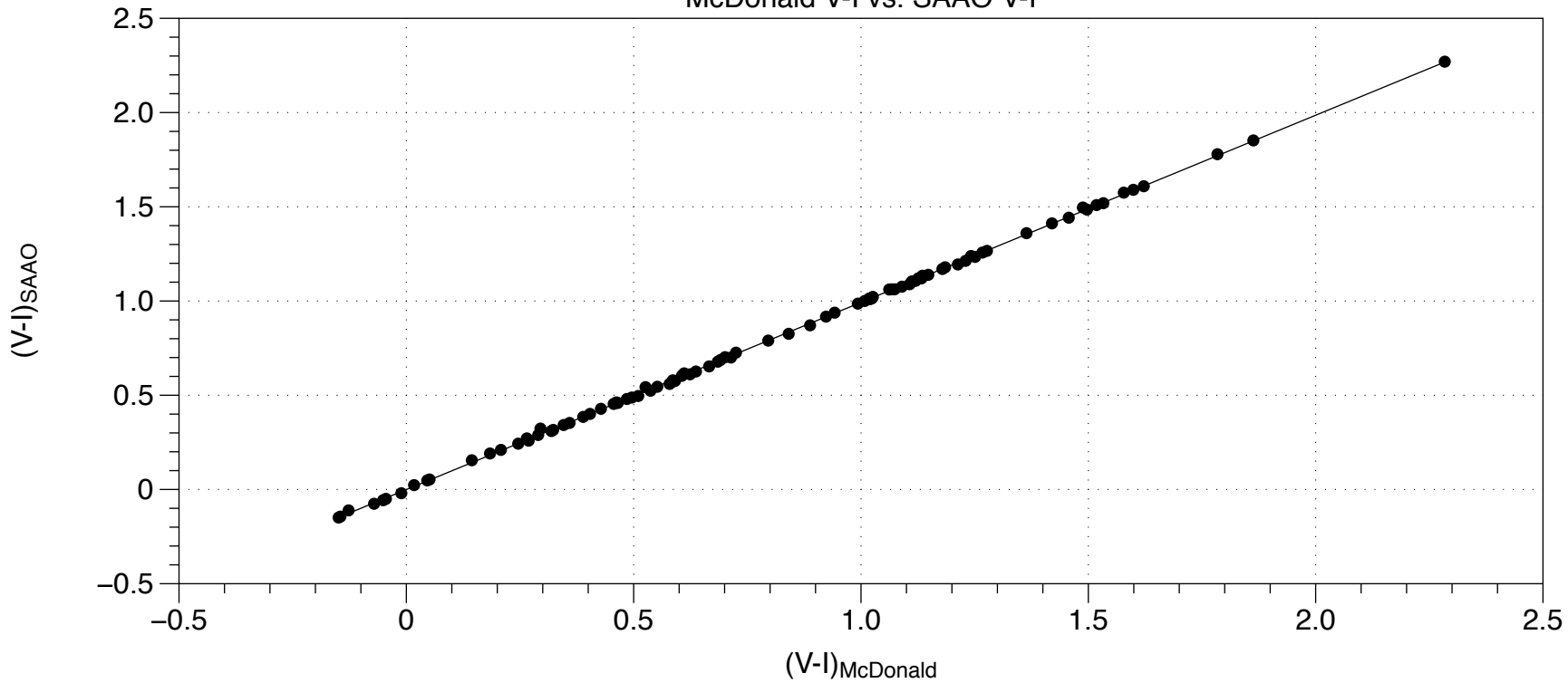
McDonald V-I vs. SAAO V-I
