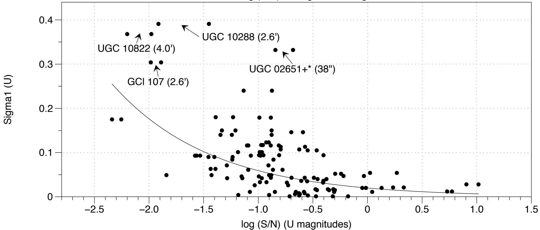
Galaxies: \log(S/N) vs. \Sigma_1 , U Magnitudes
