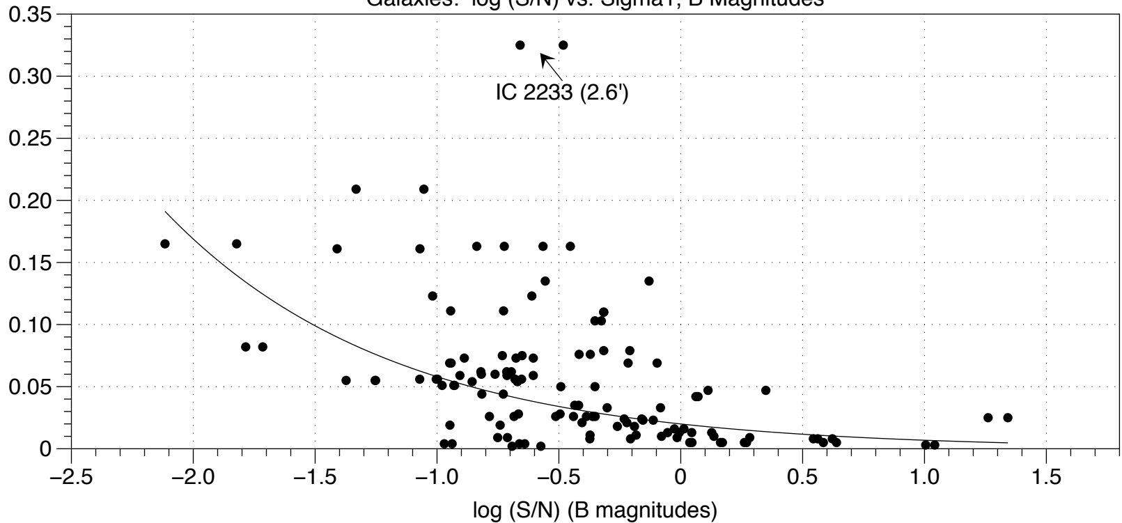
Galaxies: \log(S/N) vs. Sigma1, B Magnitudes
