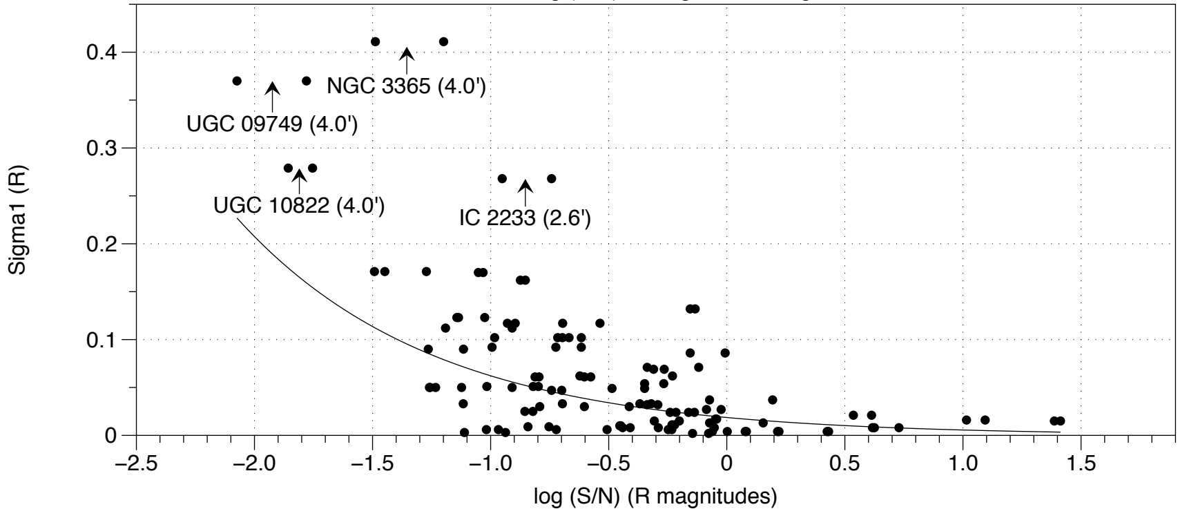
Galaxies: \log(S/N) vs. \Sigma_1 , R Magnitudes
