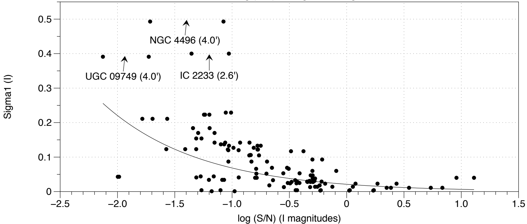
Galaxies: log (S/N) vs. Sigma1, I Magnitudes
