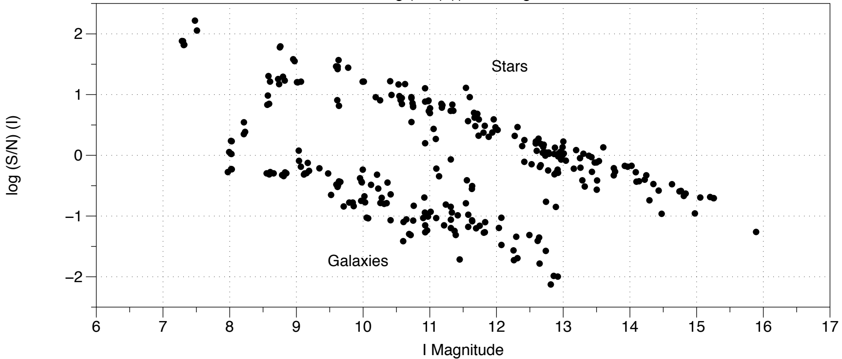
All: \log(S/N) (I) vs. I Magnitude
