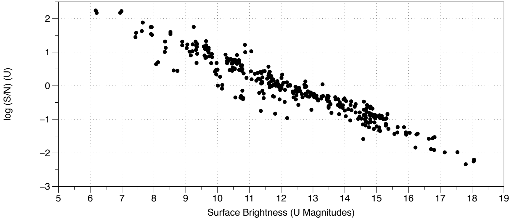
All: \log(S/N) (U) vs. Surface Brightness (U Magnitudes)
