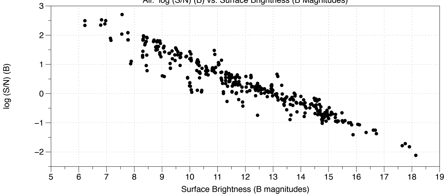
All: \log(S/N) (B) vs. Surface Brightness (B Magnitudes)
