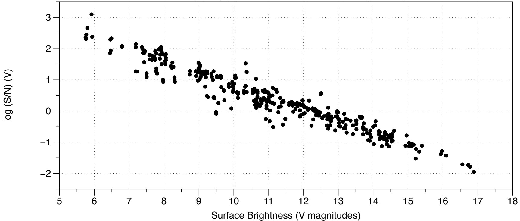
All: \log(S/N) (V) vs. Surface Brightness (V Magnitudes)
