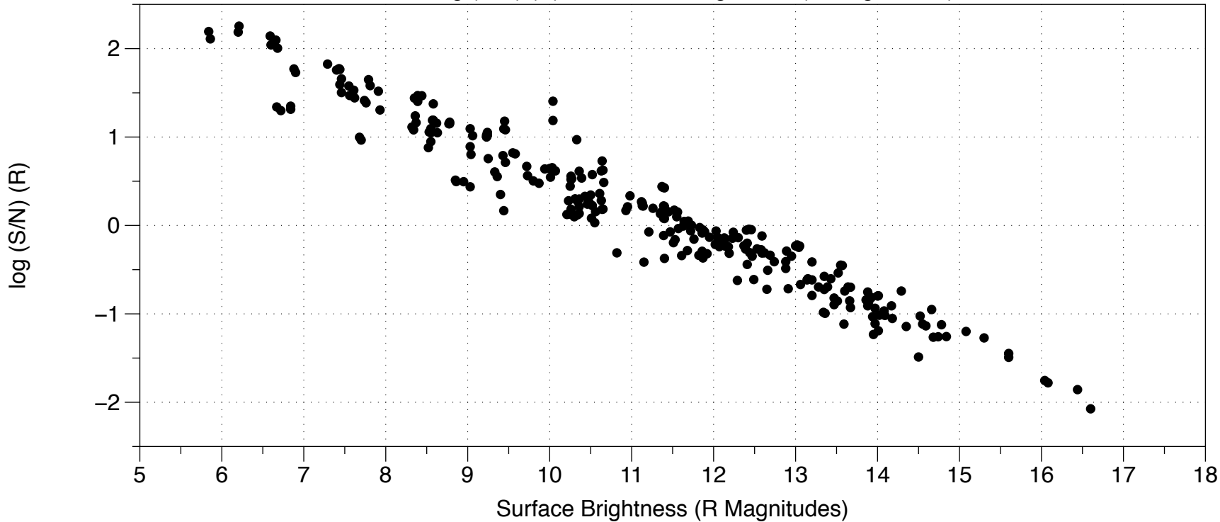
All: \log(S/N) (R) vs. Surface Brightness (R Magnitudes)
