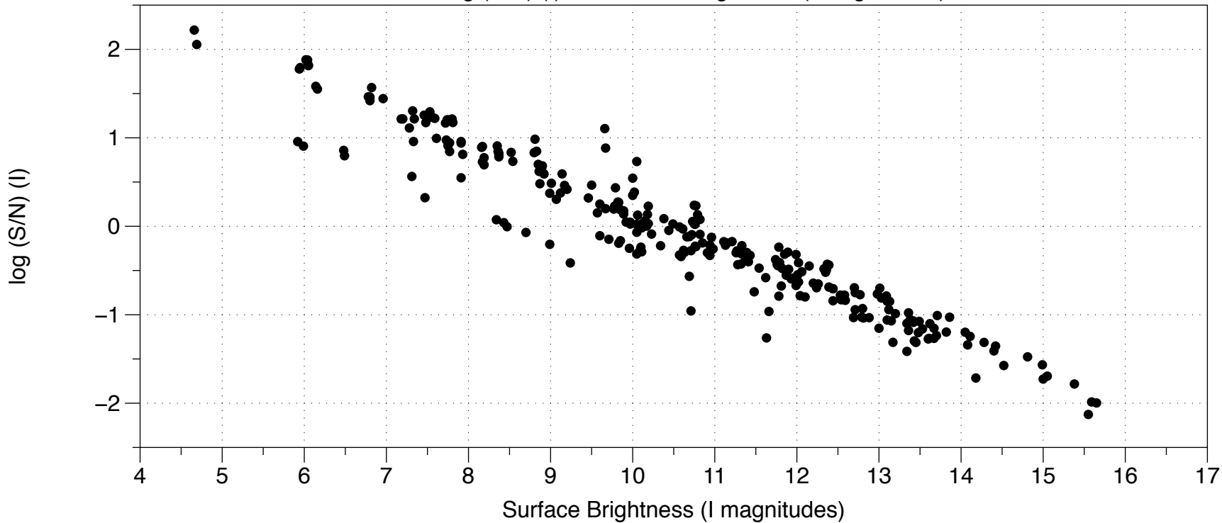
All: \log(S/N) (I) vs. Surface Brightness (I Magnitudes)
