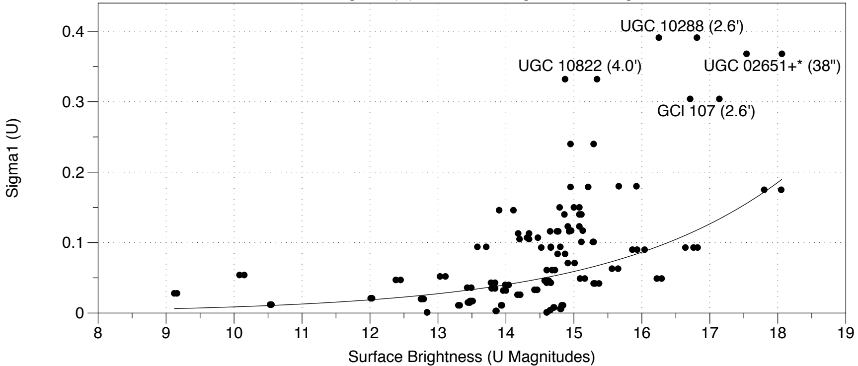
Galaxies: Sigma1 (U) vs. Surface Brightness, U Magnitudes
