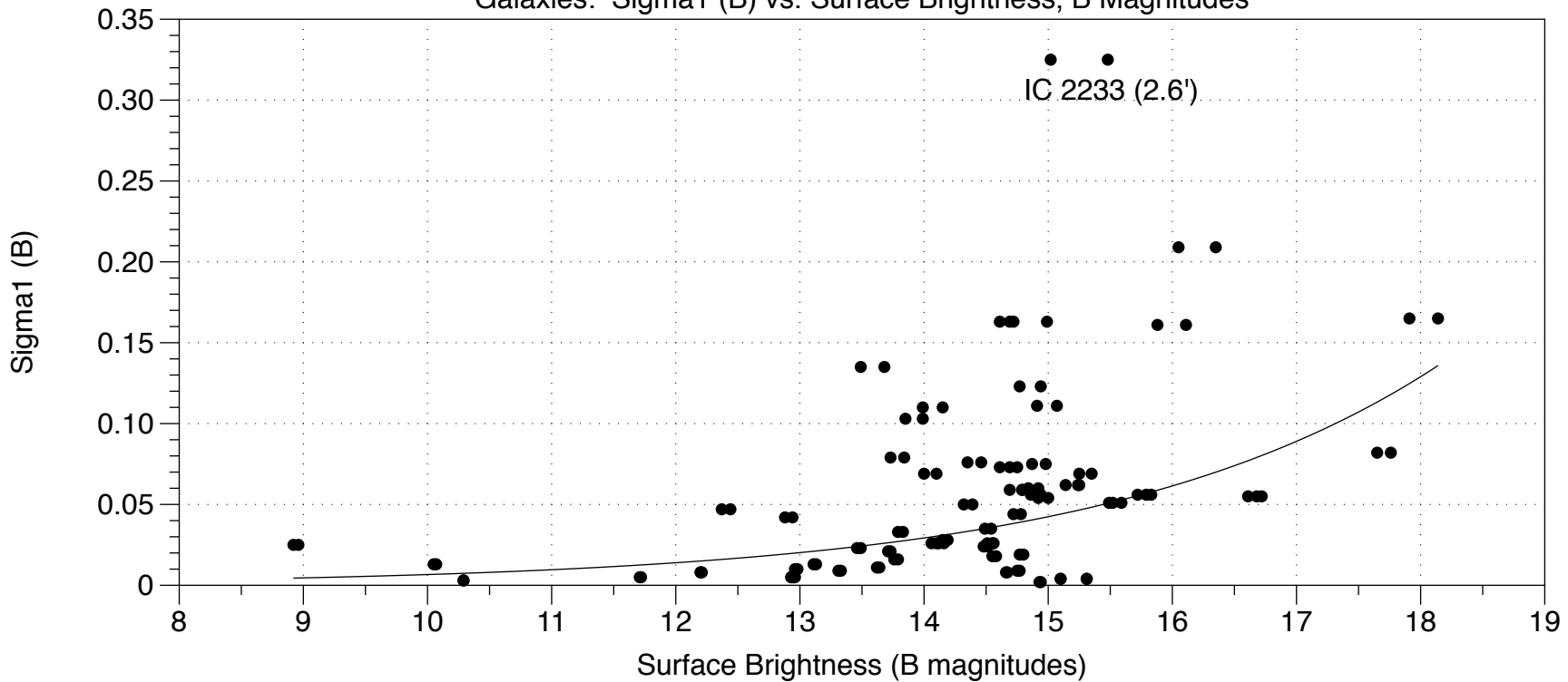
Galaxies: Sigma1 (B) vs. Surface Brightness, B Magnitudes
