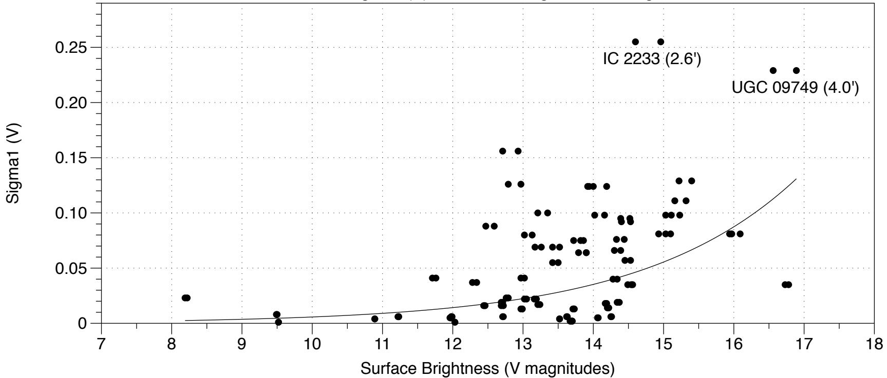
Galaxies: Sigma1 (V) vs. Surface Brightness, V Magnitudes
