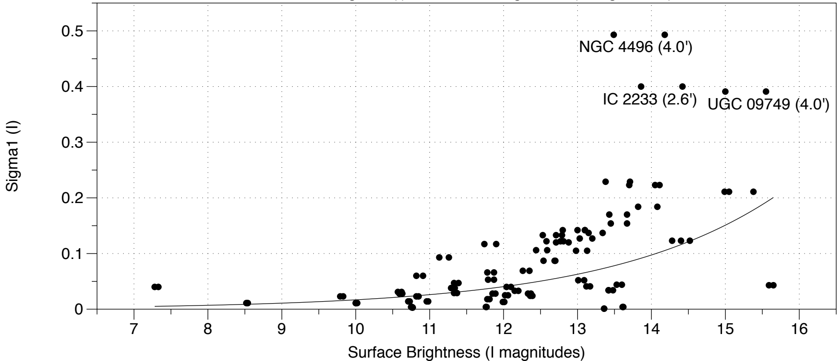
Galaxies: Sigma1 (I) vs. Surface Brightness (I Magnitudes)
